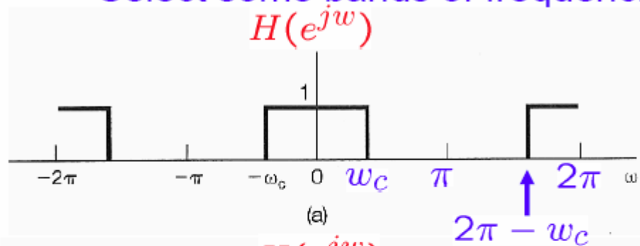
DT ideal lowpass filter
