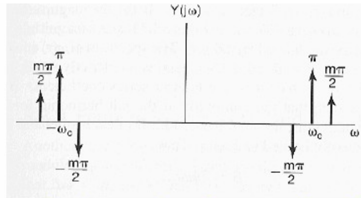
Approximate spectrum for narrowband FM
